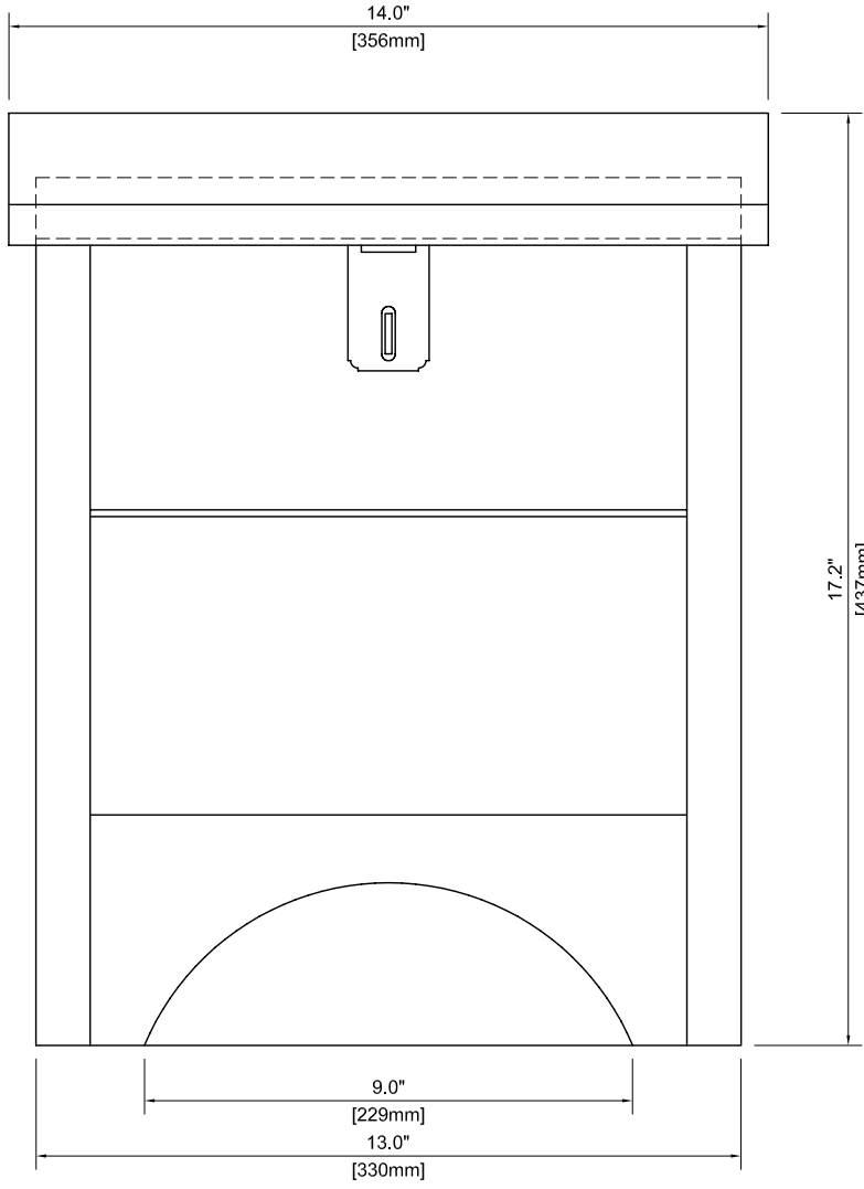
FRONT ELEVATION
