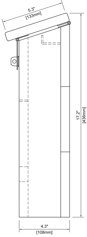
SIDE ELEVATION
